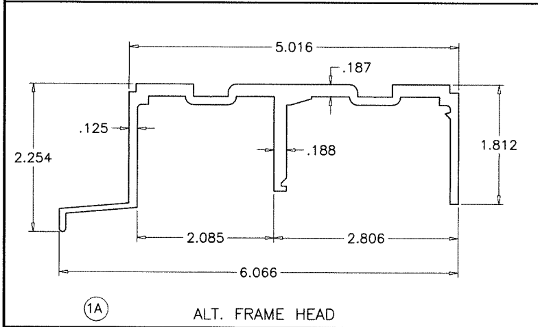
1 FRAME HEAD
