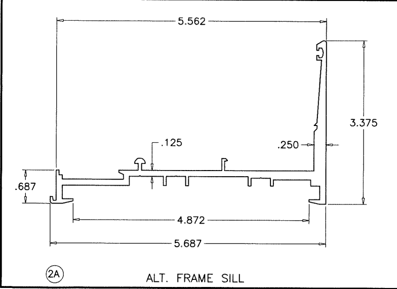
2 FRAME SILL
