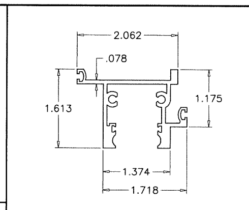
7 FIX. TOP RAIL
